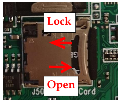
Micro SD card inserted and locked
